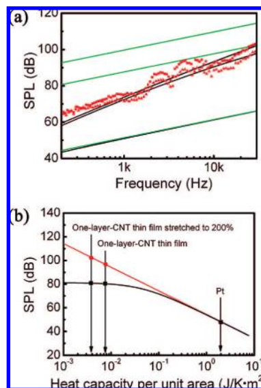
Figure 5. Theoretical and experimental data for the thermoacoustic thin film loudspeakers. (a) Theoretical and experimental results of the SPLs versus frequency of thermoacoustic thin film loudspeakers. The experimental data are represented by red solid squares and triangles for one-layer and four-layer CNT thin films, respectively. The green lines and black lines are SPLs calculated according to Arnold and Crandall’s theory (eq 1) and our theory (eq 2), respectively, for one-layer (upper) and four-layer (middle) CNT loudspeakers and a 700 nm thick Pt thermophone (lower). The input powers are all 4.5 W. (b) The dependence of SPLs (at 10 KHz with input power 1 W) on HCPUA C_s is calculated according to Arnold and Crandall’s theory (eq 1, red line) and our theory (eq 2, black line), respectively.
