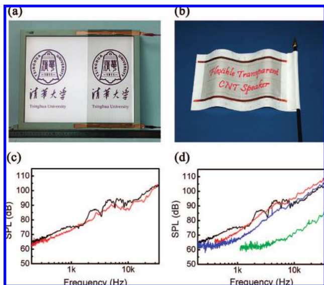
Figure 4. Transparent, flexible, CNT thin film loudspeaker. (a) A transparent CNT thin film loudspeaker is directly mounted on the frame of a 17 in. LCD screen. (b) The CNT thin film was put on a flag to make a flexible flag loudspeaker with dimensions of 8 cm by 14.5 cm. (c) Measured SPLs versus frequency for a one-layer CNT thin film that is either freestanding (black) or put on a piece of cloth (red). Both input powers are 4.5 W. (d) Measured SPLs versus frequency for a one-layer CNT thin film when it is freestanding (black), put on a ground glass (red), put on window glass (blue), or put on window glass with further ethanol treatment (green). The process of ethanol treatment is as follows: drop and spread some ethanol on the window glass covered by CNT thin films, then wait until the ethanol evaporates. All the input powers are 4.5 W.
